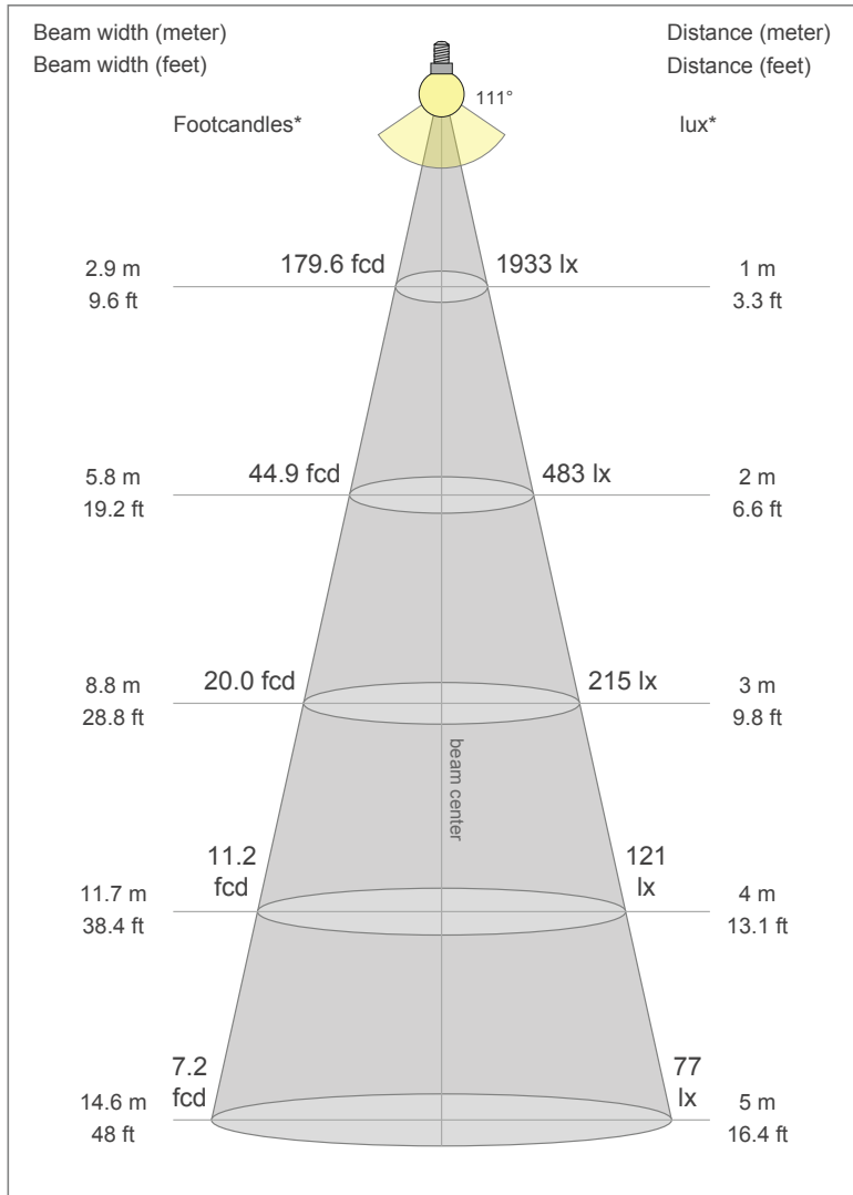
Beam Details
